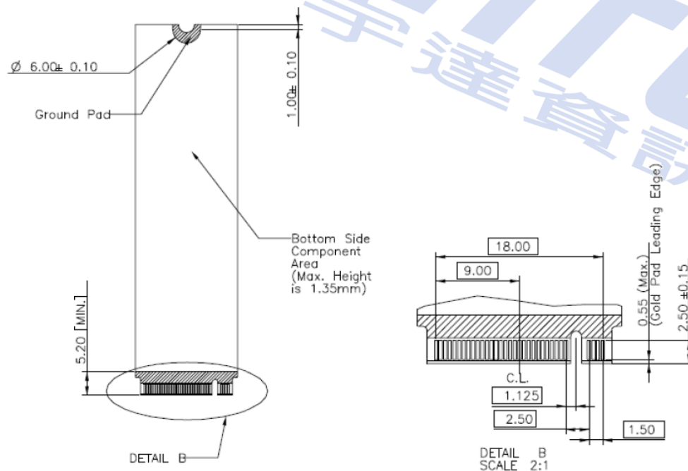
Bottom View
